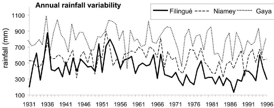
Figure 1 - Annual Rainfall Trends in Niger from 1950 - 1996
